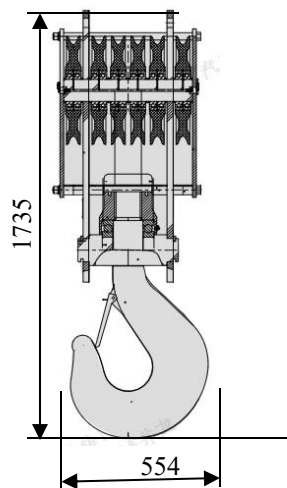
85t钩 85 t hook block
