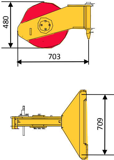
臂端单滑轮 95kg Single top (auxiliary sheave)
