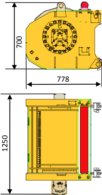
副起升机构 (含钢丝绳) 900kg Auxiliary winch (rope included)
