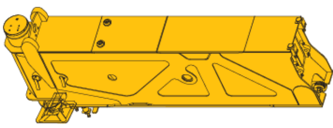
后活动支腿 1280kg Rear outrigger beam 1280kg 2550×1290×395
